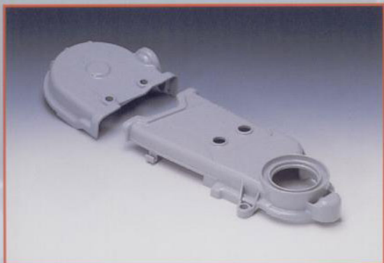
CIVIC 79 COVER COMP., TIMING BELT SK1421-CV79 11811-634-000 (LOWER) SK1422-CV79 11812-634-000 (UPPER)
