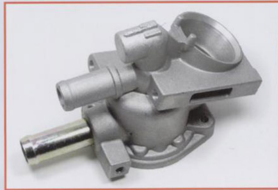
CR-V 97 RD1 節溫器座 CASE COMP., THERMOSTAT SK1512-CRV97 19320-P30-000
