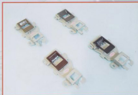
CIVIC 88-91,COLORS HANDLE ASSY., INSIDE F.(POWER) SK6111-CV88 72120-SH4-A21 (RH) SK6112-CV88 72160-SH4-A21 (LH)
