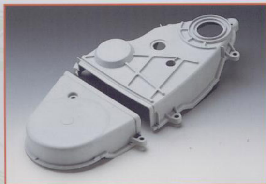
CIVIC 84-87 COVER COMP., TIMING BELT SK1421-CV84 11810-PEO-020 (LOWER) SK1422-CV84 11820-PEO-000 (UPPER)
