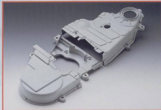
CIVIC 88-95 COVER COMP., TIMING BELT SK1421-CV88 11810-PM3-000 (LOWER) SK1422-CV88 11820-PM3-000 (UPPER) SK1424-CV88 11840-PM3-000 (BACK)
