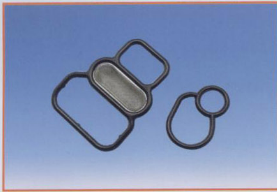
CIVIC 96 VTEC 電磁閥墊片 FILTER ASSY., SPOOL VALVE SK1921-CV96-UP 36172-PO8-015 (SMALL) SK1921-CV96-LOW 15825-P2M-005 (LARGE)
