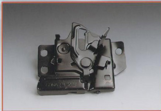
CIVIC 92-97, CITY 96 引擎蓋六角鎖EK3 LOCK ASSY., HOOD SK6273-CV92 74120-SO4-A01 SK6273-CTY96 74120-SX8-T01
