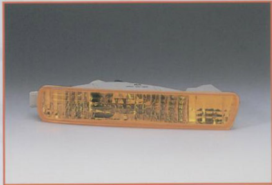
ACCORD 94 保桿小燈 FRONT LAMP SK3311-ACD94 33300-SV4-A01 (RH) SK3312-ACD94 33350-SV4-A01 (LH) 40PCS/4.14'
