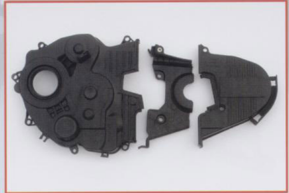
ACCORD98-廣本2.3/CG5 COVER COMP.,TIMING BELT SK1421-ACD98 11810-PAA-T00 (LOWER) SK1422-ACD98 11820-POA-000 (UPPER) SK1424-ACD98 11830-POA-020 (BACK)
